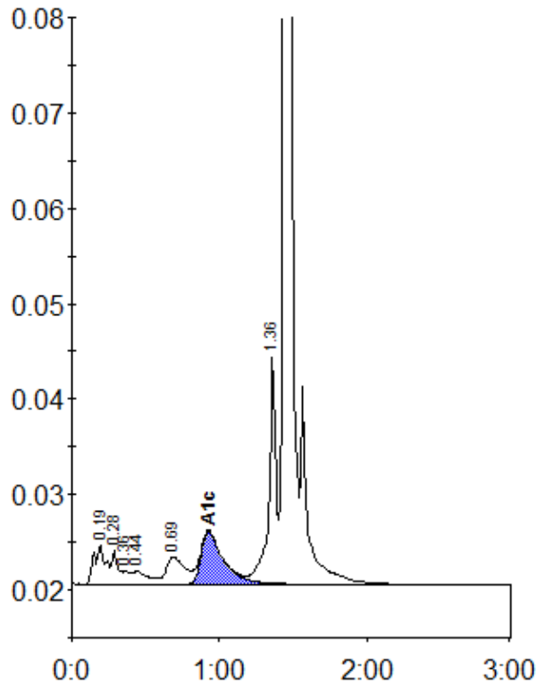
Peak table - ID: 10448390
